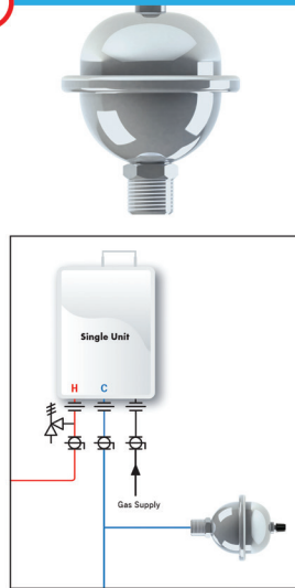
ZEP-1 can be installed below the isolation kit or anywhere on the cold water supply line between the heater and the check valve.
